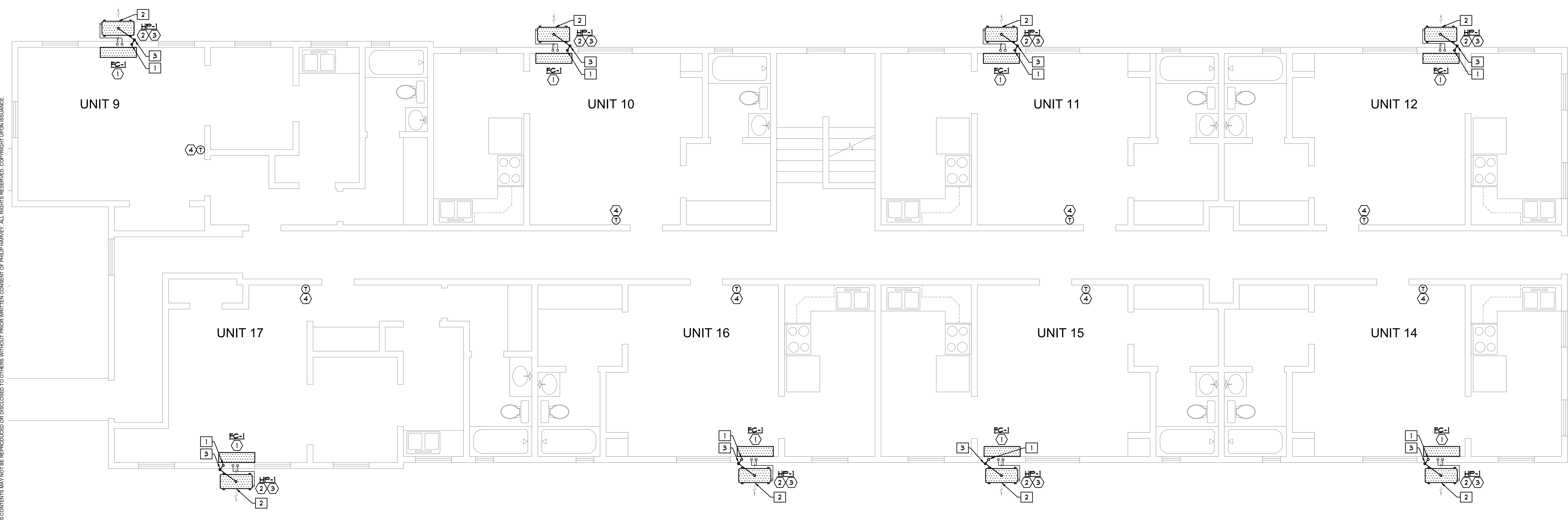
MECHANICAL SECOND FLOOR PLAN SCALE: 1/4"=1'-0"
