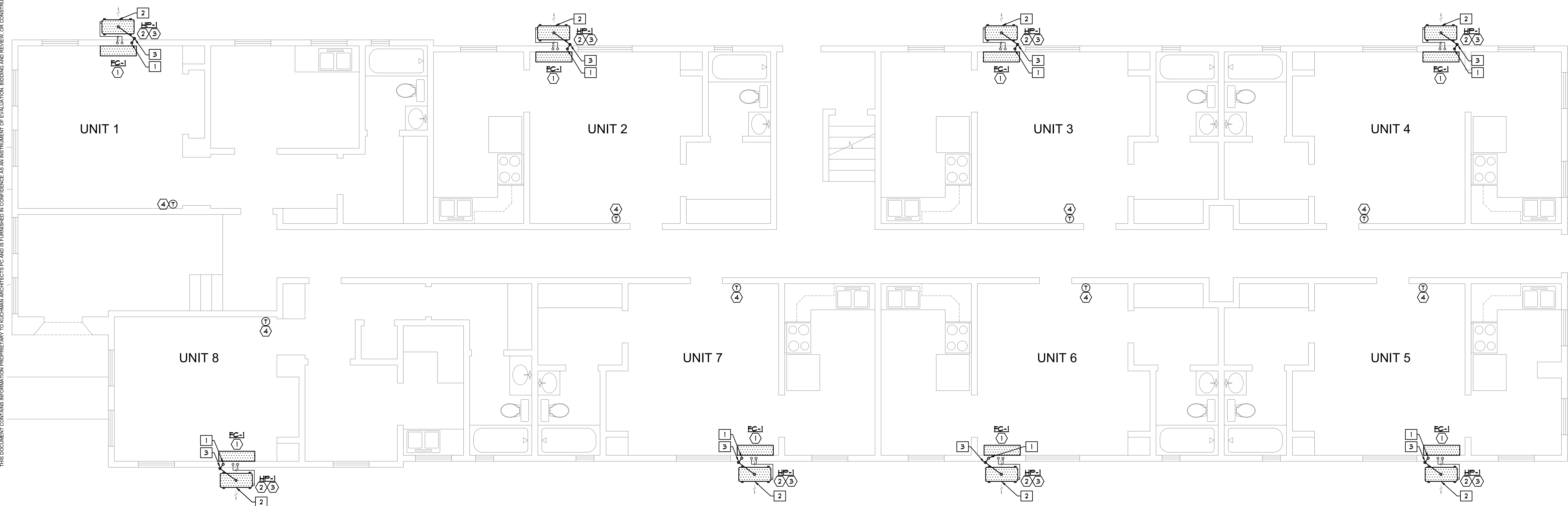
MECHANICAL FIRST FLOOR PLAN SCALE: 1/4"=1'-0"
