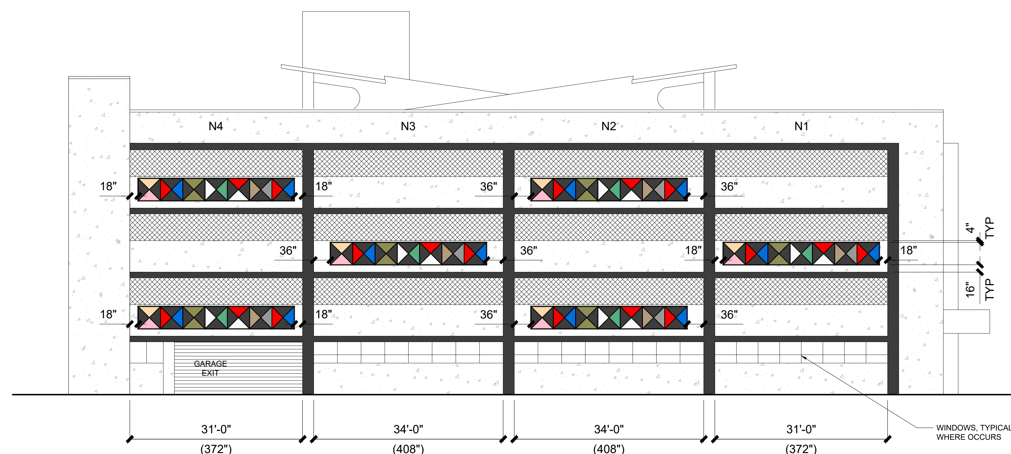
3 EXTERIOR ELEVATION - 9TH STREET (WEST) A3.1 SCALE 3/32" = 1'-0"
