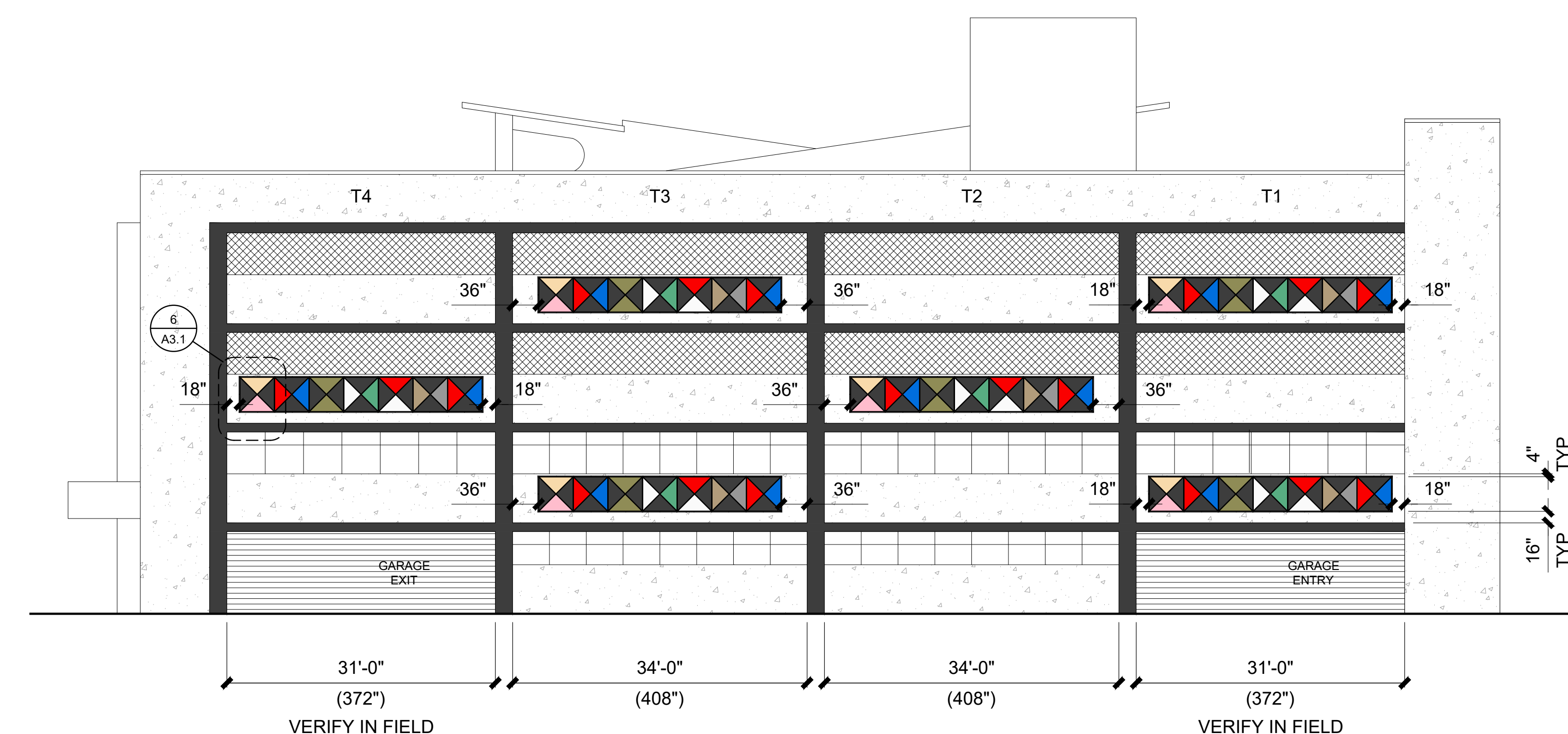
2 A3.1 EXTERIOR ELEVATION - 10TH STREET (EAST) SCALE 3/32" = 1'-0"
